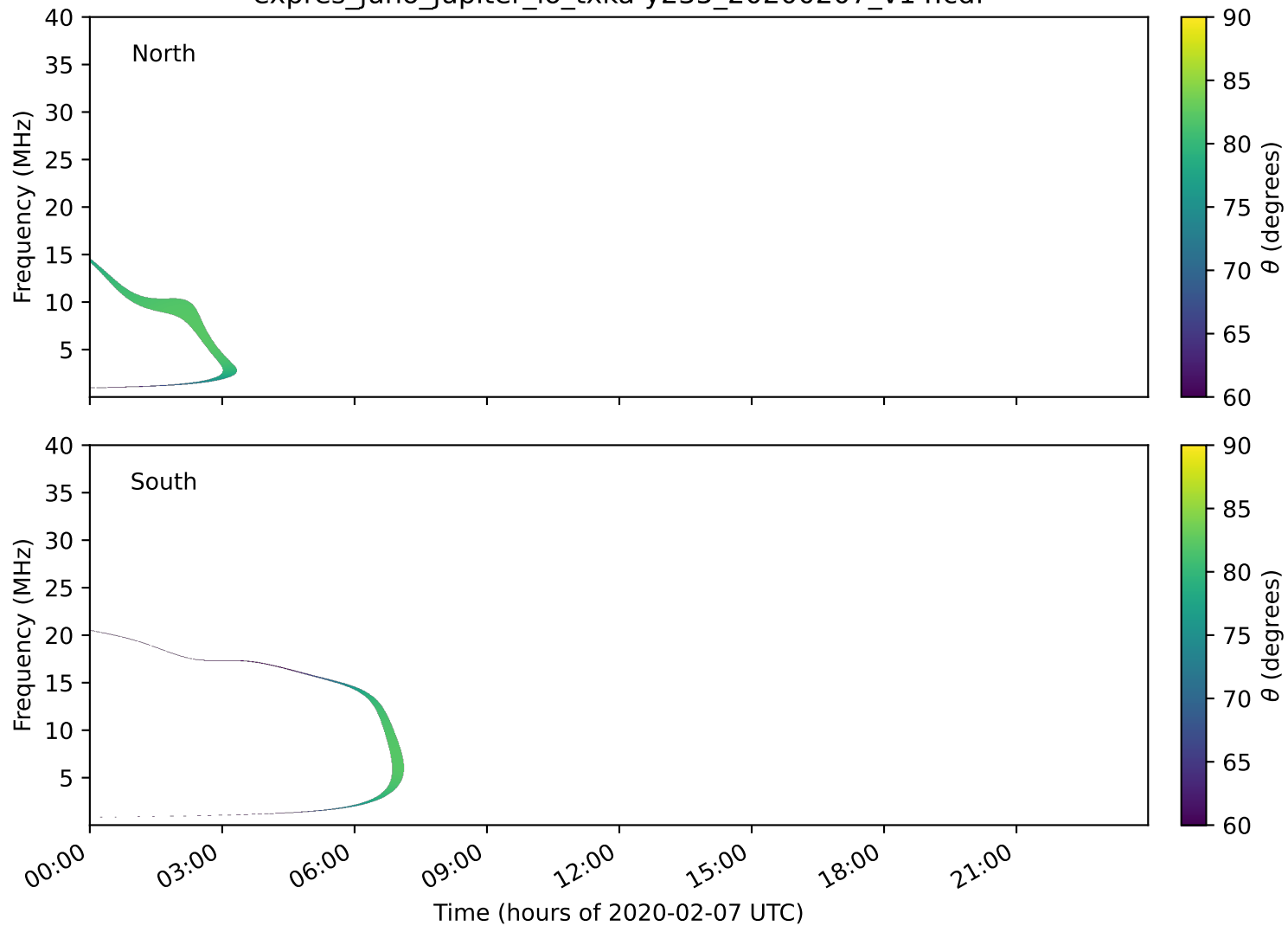
expres_juno_jupiter_io_txka-y235_20200207_v14.cdf
