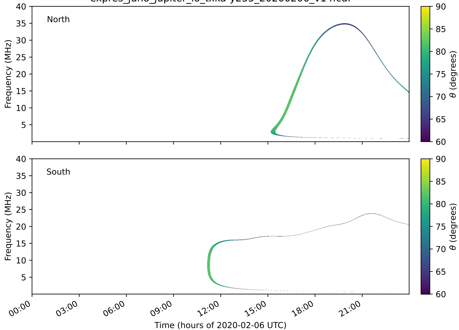
expres_juno_jupiter_io_txka-y235_20200206_v14.cdf
