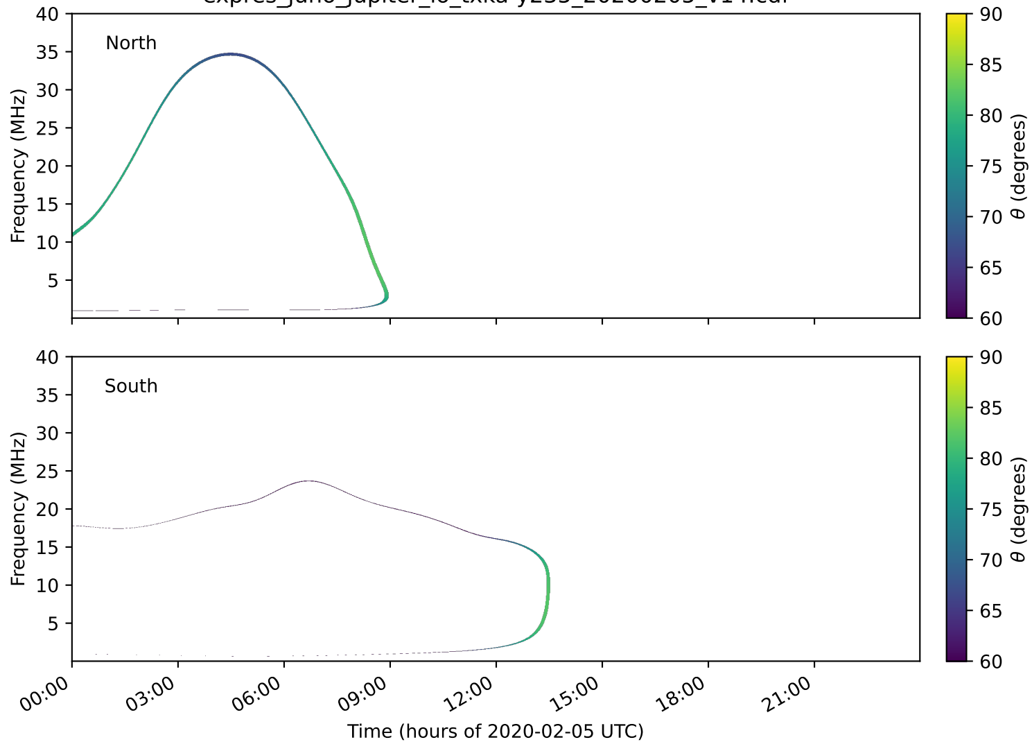
expres_juno_jupiter_io_txka-y235_20200205_v14.cdf
