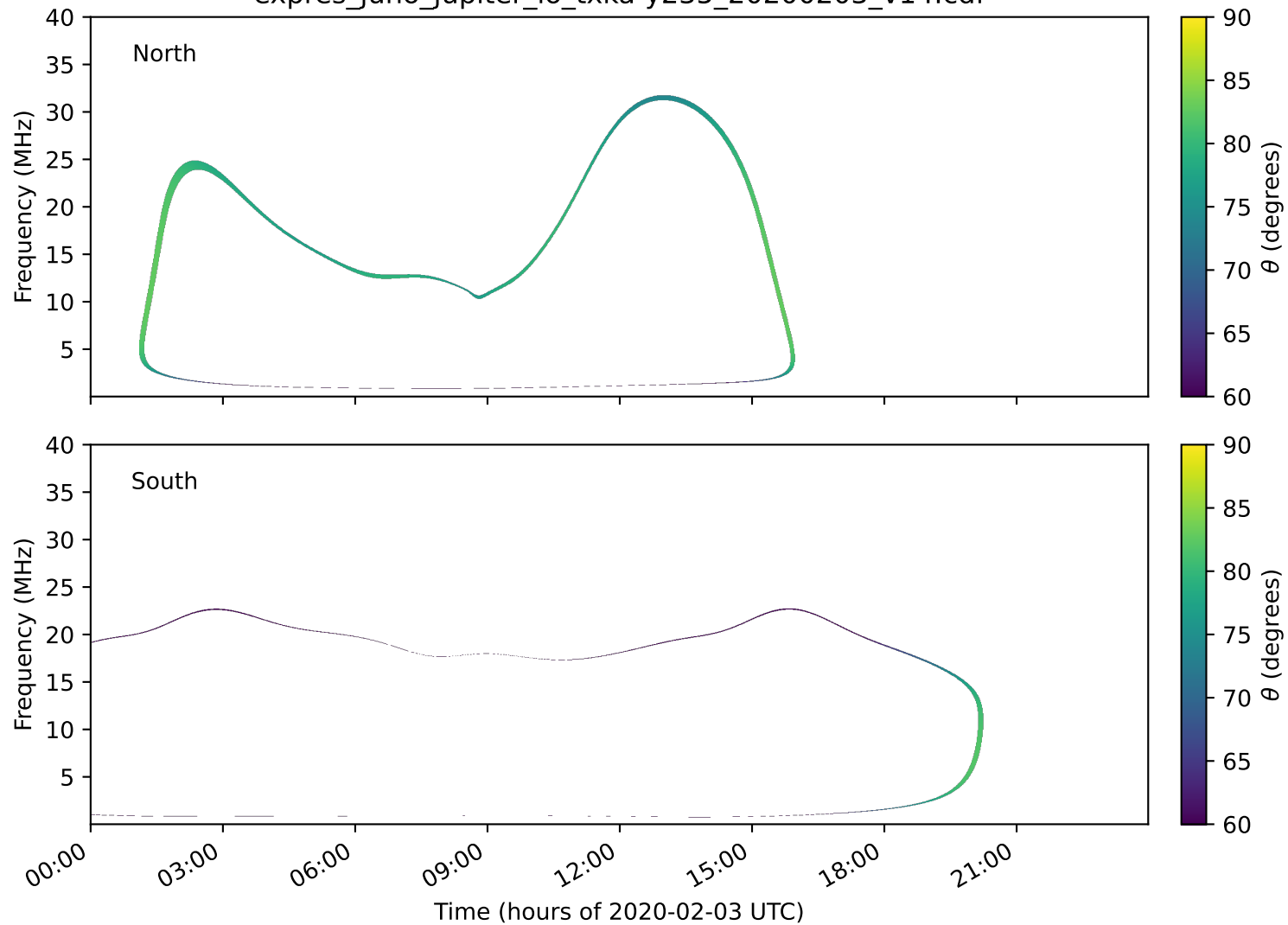
expres_juno_jupiter_io_txka-y235_20200203_v14.cdf
