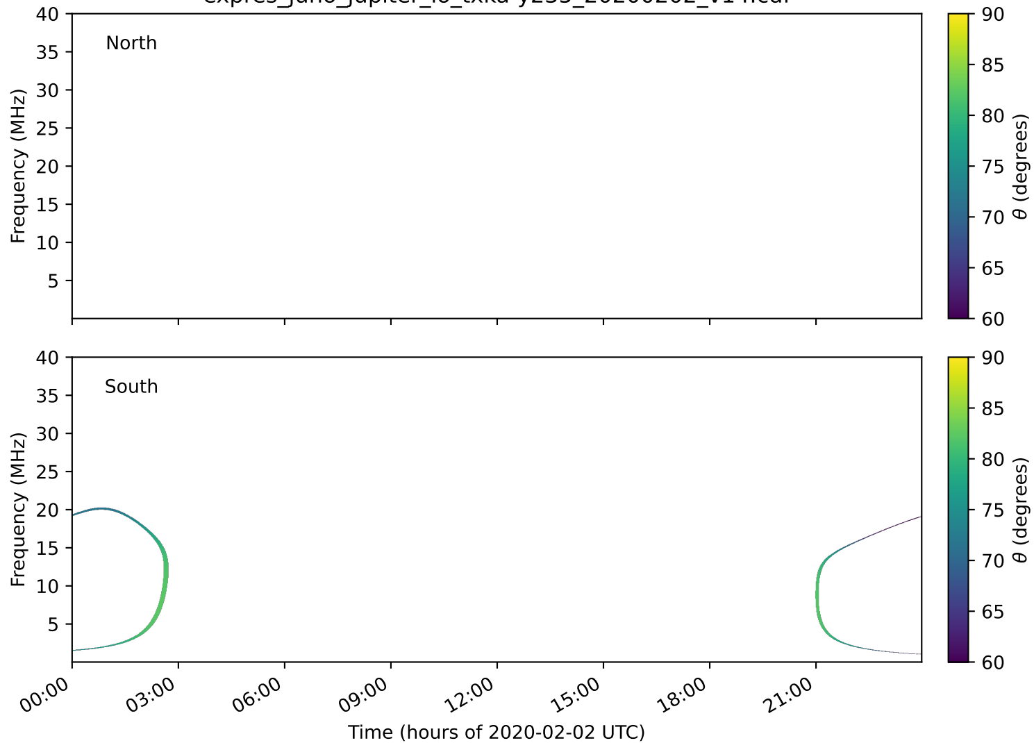
expres_juno_jupiter_io_txka-y235_20200202_v14.cdf
