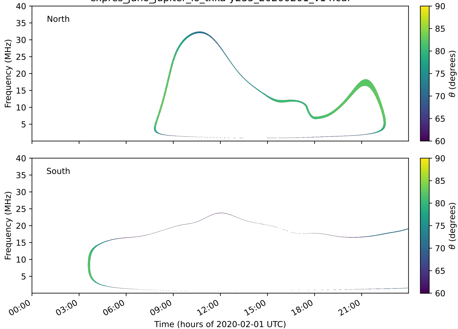
expres_juno_jupiter_io_txka-y235_20200201_v14.cdf
