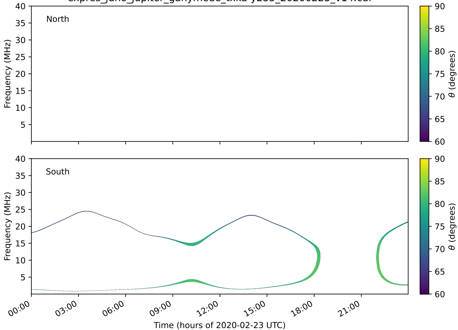
expres_juno_jupiter_ganymede_txka-y235_20200223_v14.cdf
