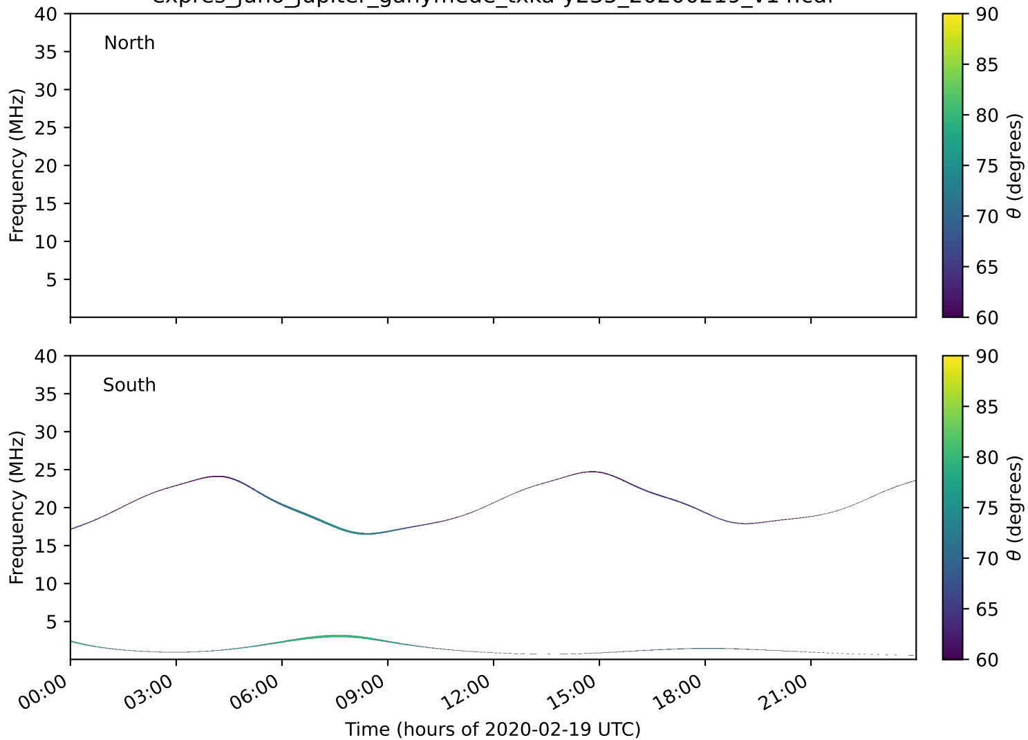
expres_juno_jupiter_ganymede_txka-y235_20200219_v14.cdf
