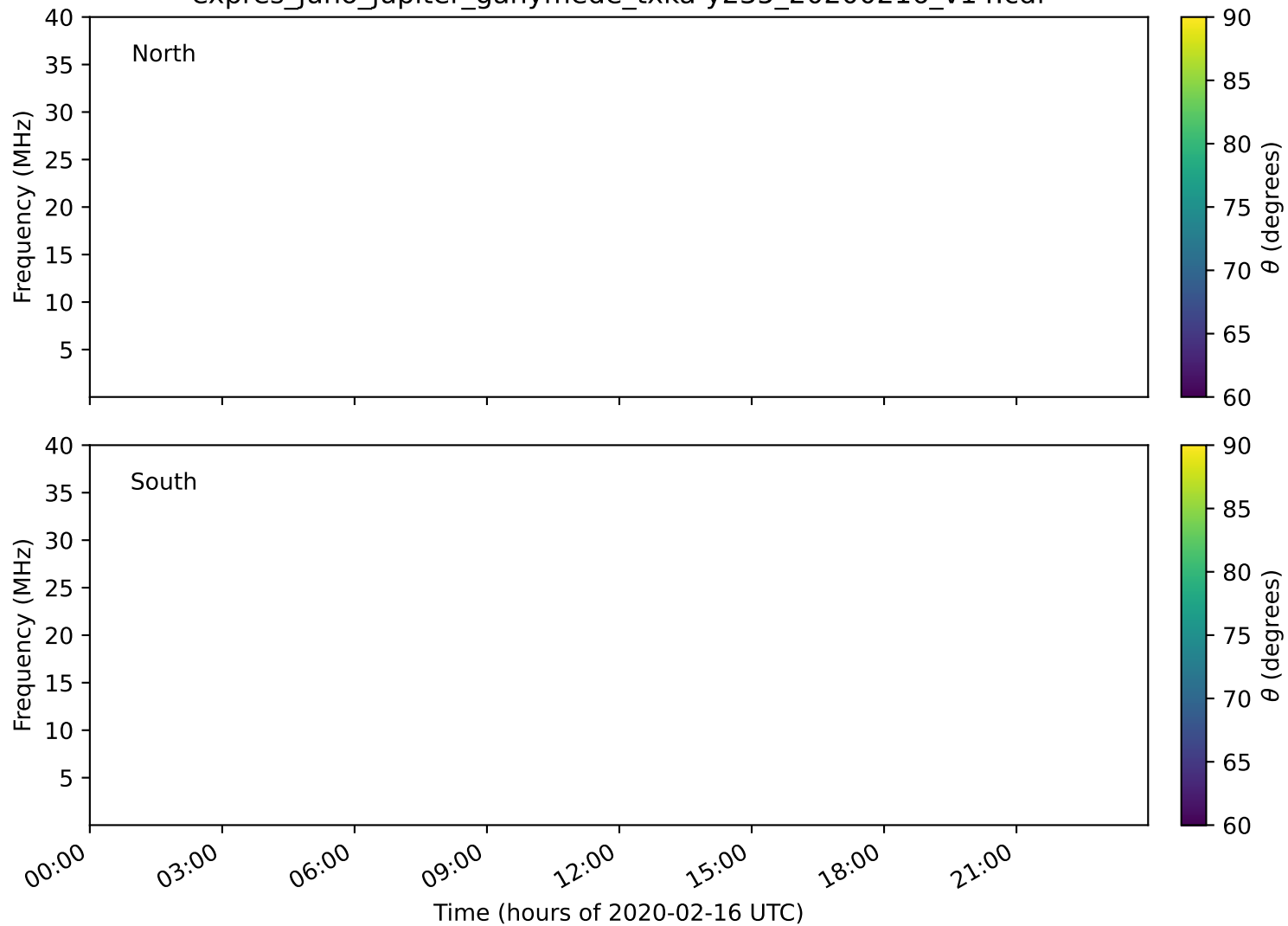
expres_juno_jupiter_ganymede_txka-y235_20200216_v14.cdf
