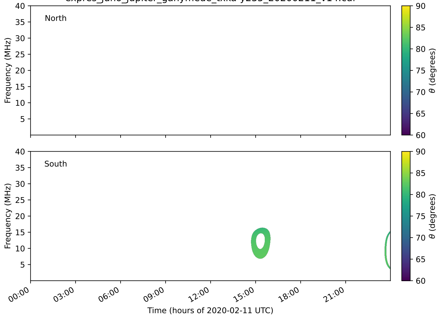
expres_juno_jupiter_ganymede_txka-y235_20200211_v14.cdf
