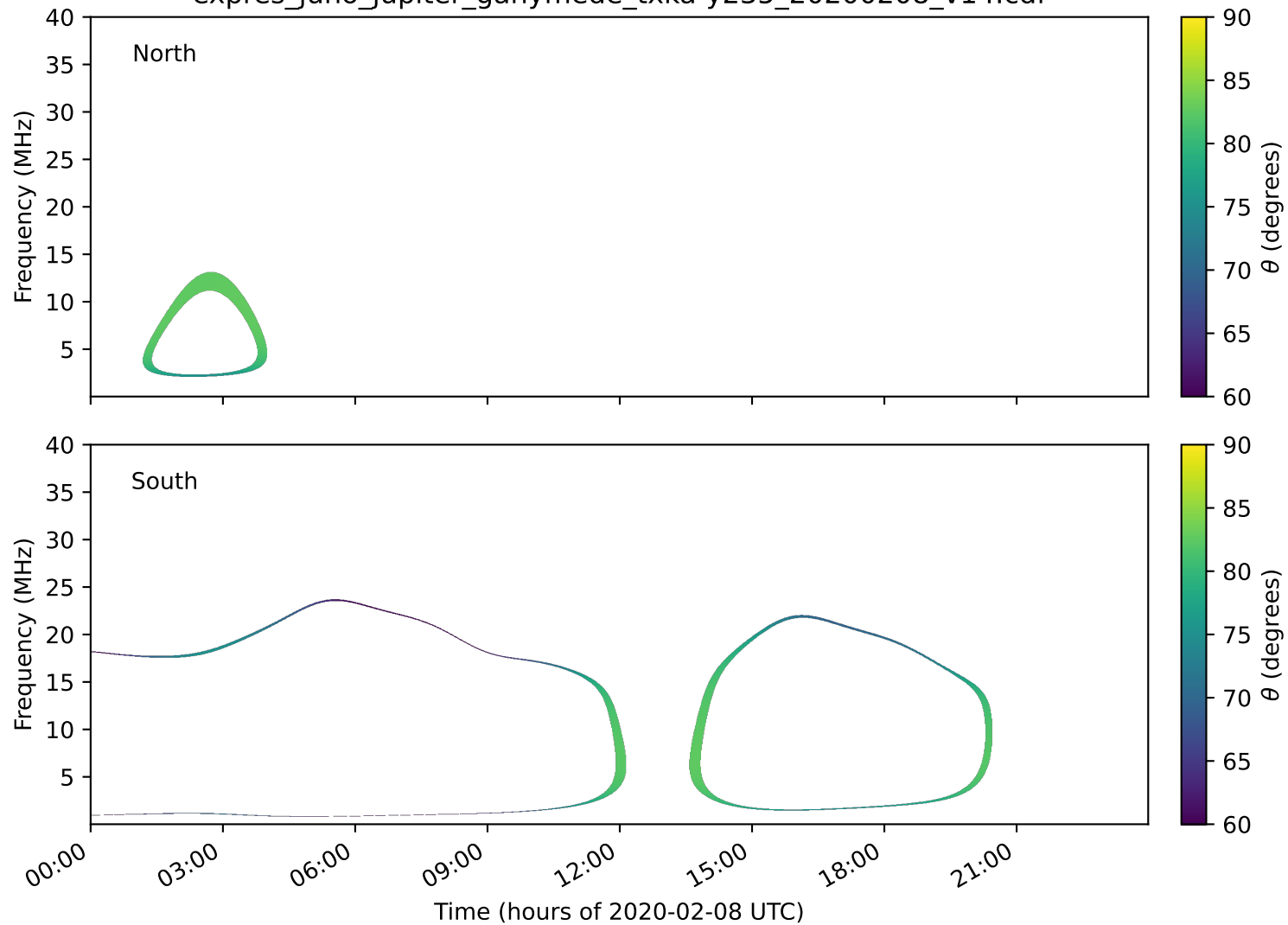
expres_juno_jupiter_ganymede_txka-y235_20200208_v14.cdf
