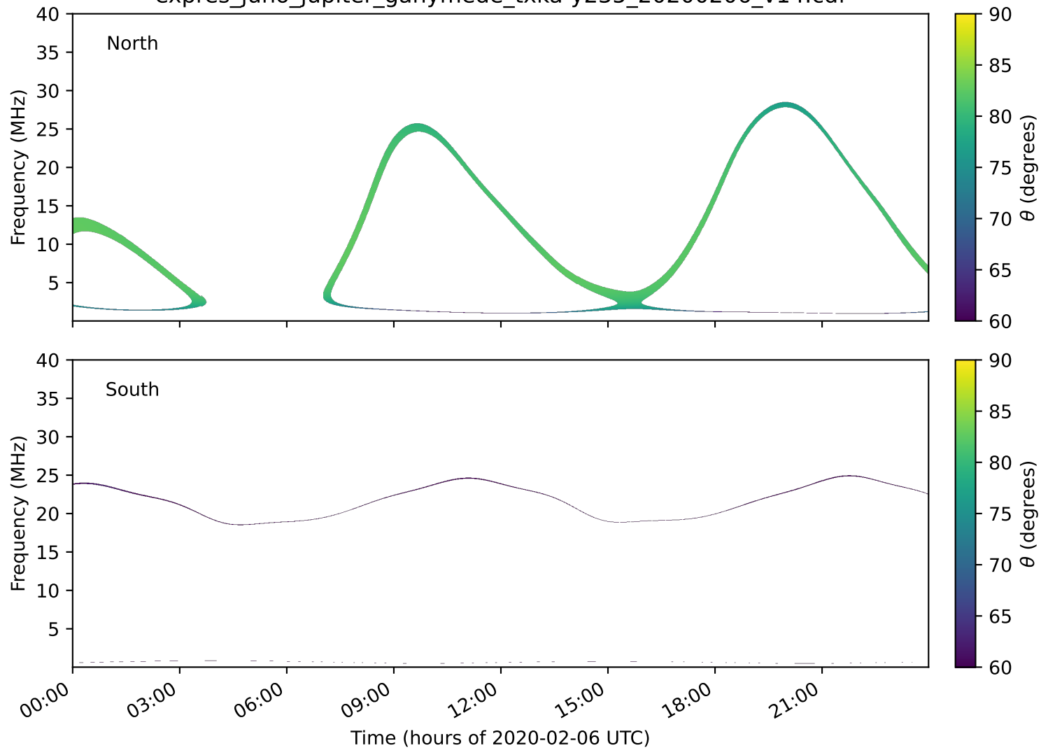
expres_juno_jupiter_ganymede_txka-y235_20200206_v14.cdf
