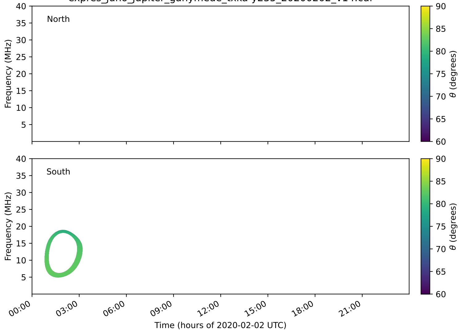
expres_juno_jupiter_ganymede_txka-y235_20200202_v14.cdf
