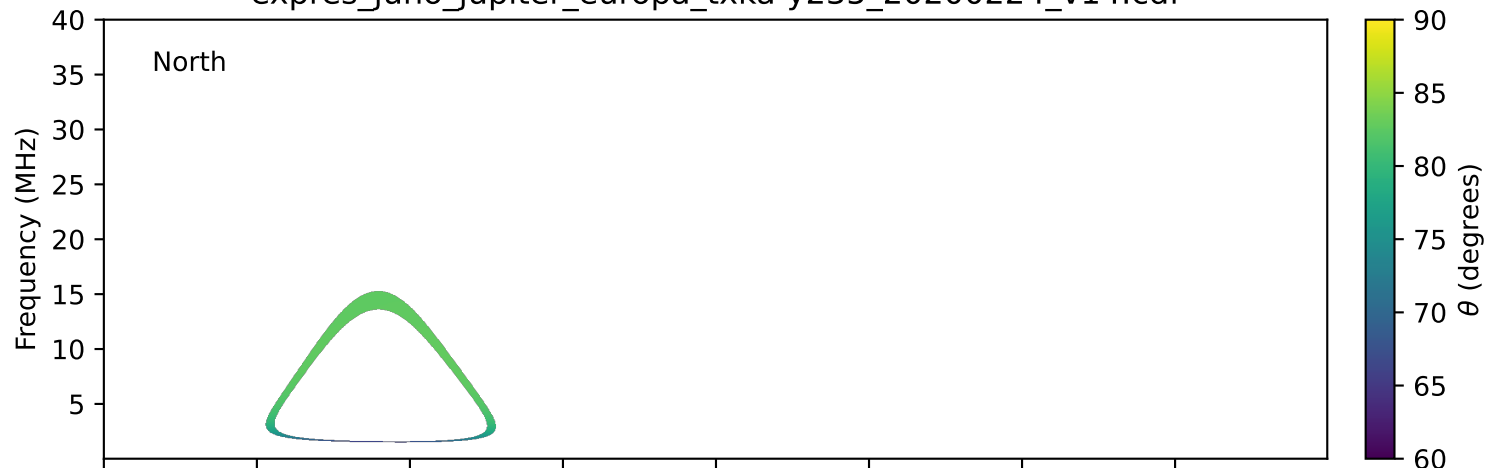
expres_juno_jupiter_europa_txka-y235_20200224_v14.cdf
