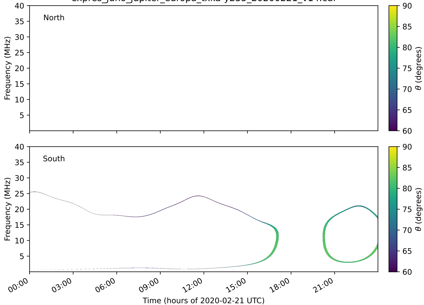
expres_juno_jupiter_europa_txka-y235_20200221_v14.cdf
