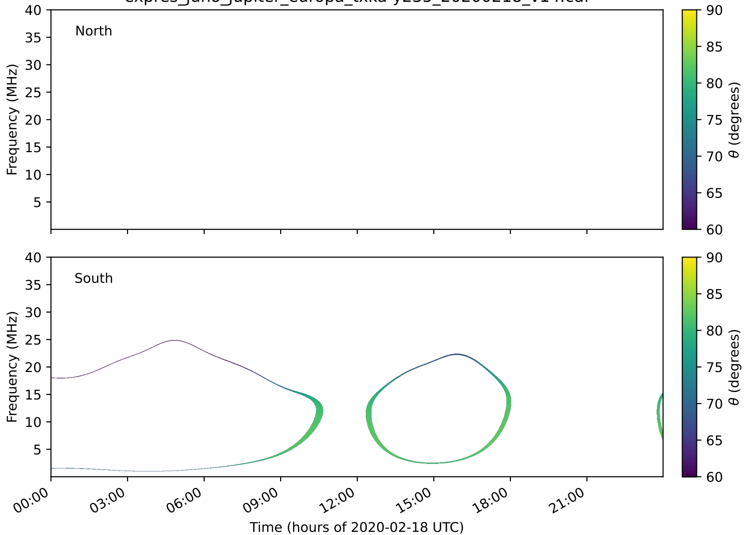
expres_juno_jupiter_europa_txka-y235_20200218_v14.cdf
