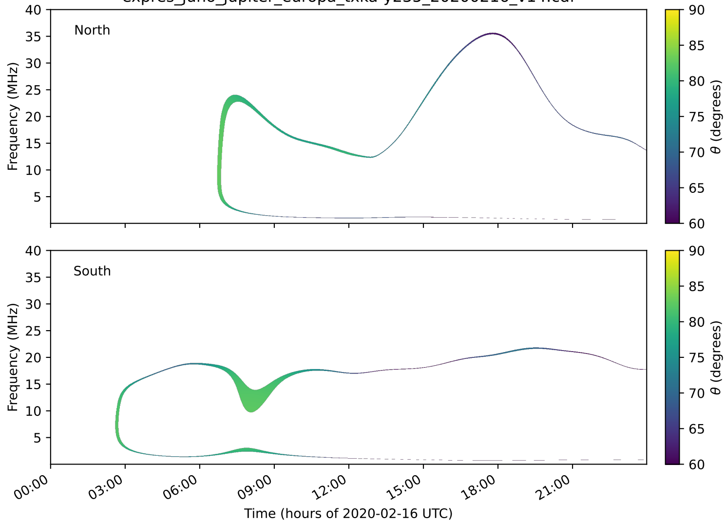
expres_juno_jupiter_europa_txka-y235_20200216_v14.cdf
