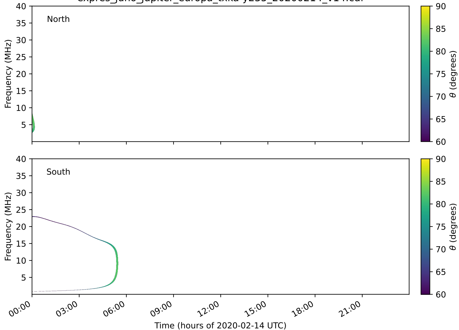
expres_juno_jupiter_europa_txka-y235_20200214_v14.cdf
