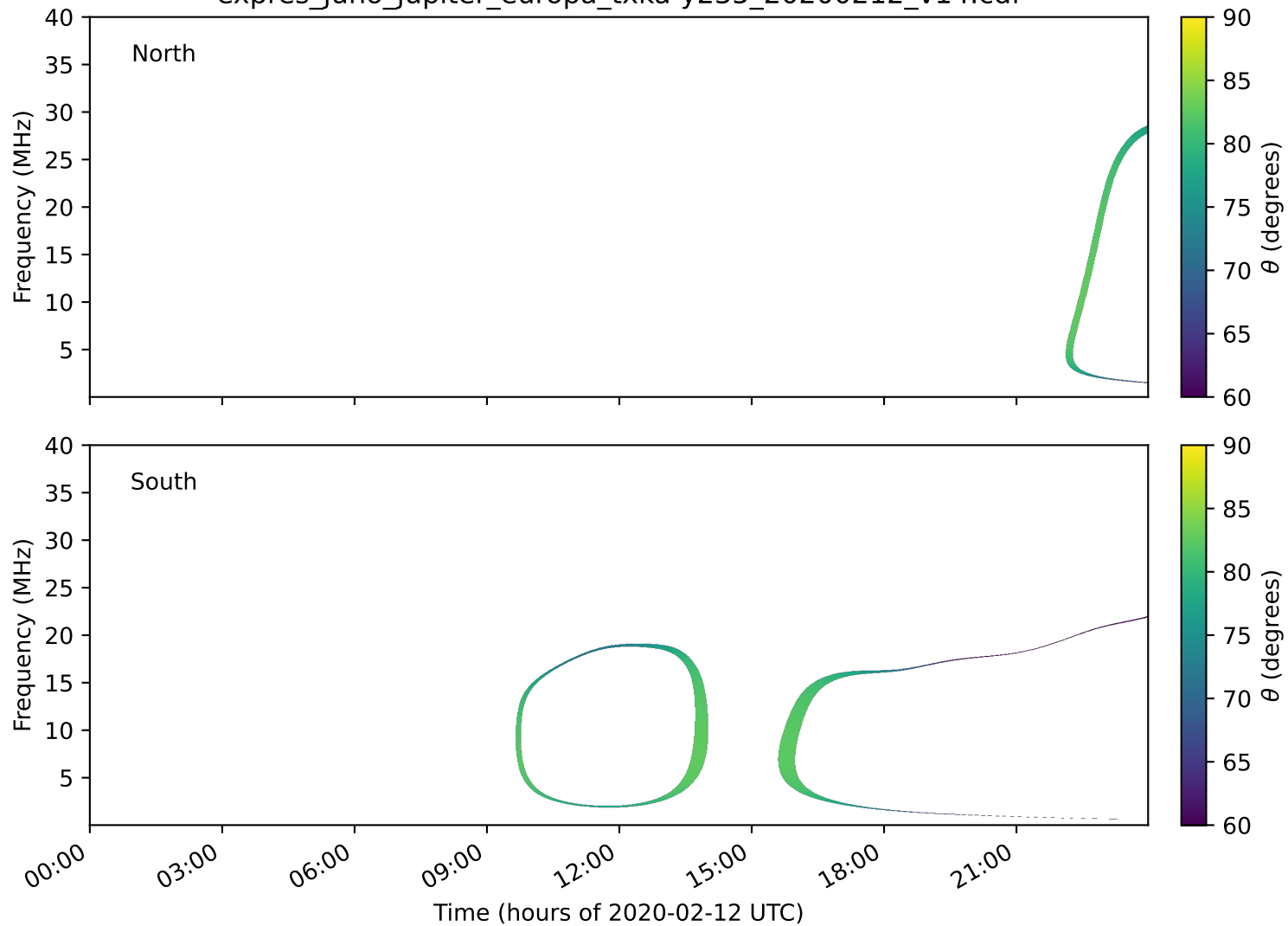
expres_juno_jupiter_europa_txka-y235_20200212_v14.cdf
