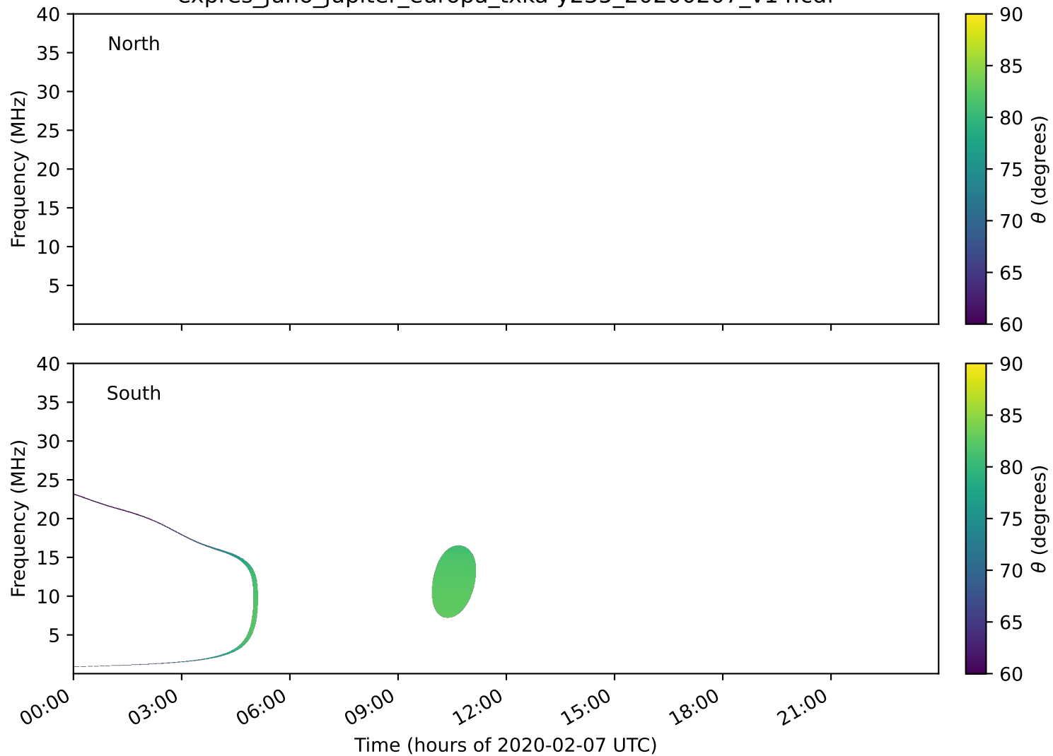
expres_juno_jupiter_europa_txka-y235_20200207_v14.cdf
