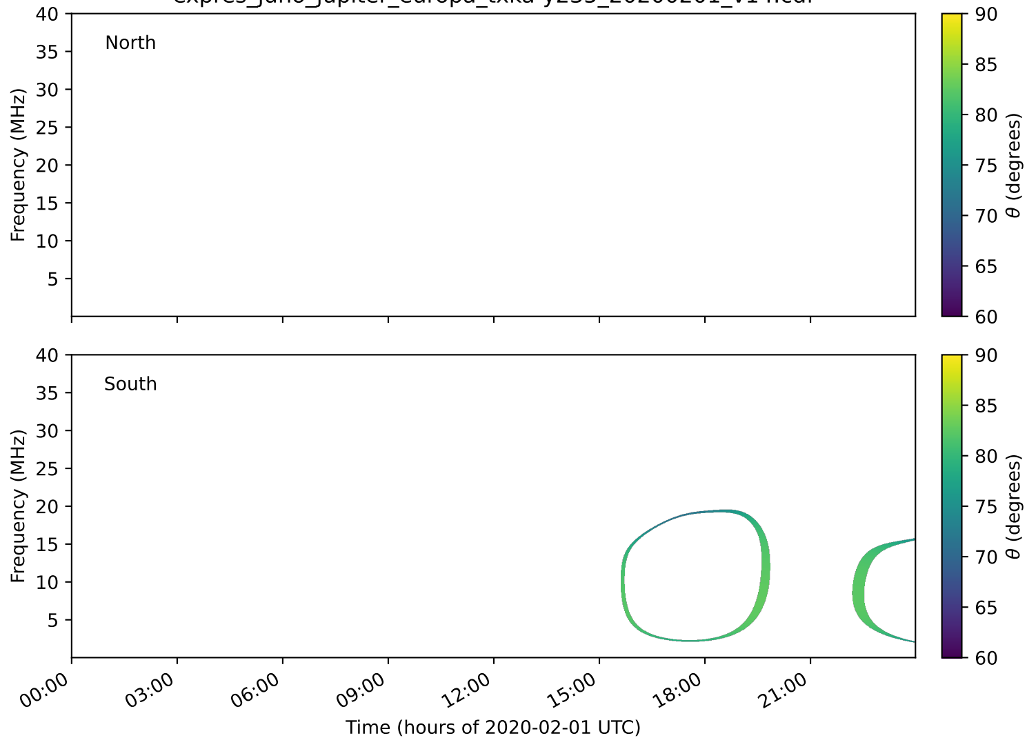
expres_juno_jupiter_europa_txka-y235_20200201_v14.cdf
