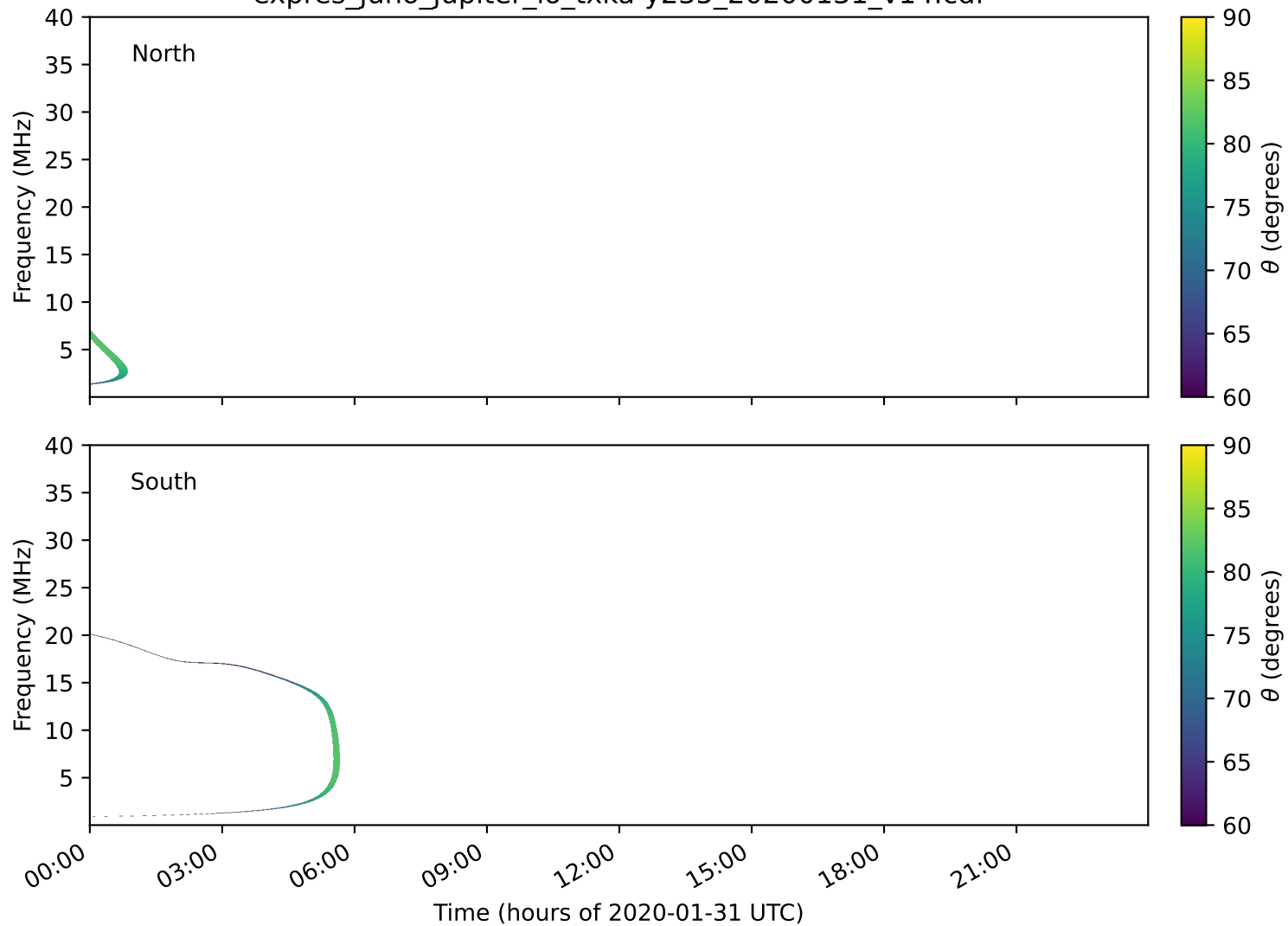
expres_juno_jupiter_io_txka-y235_20200131_v14.cdf
