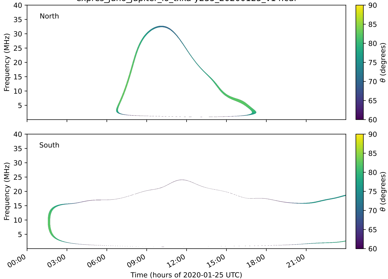
expres_juno_jupiter_io_txka-y235_20200125_v14.cdf
