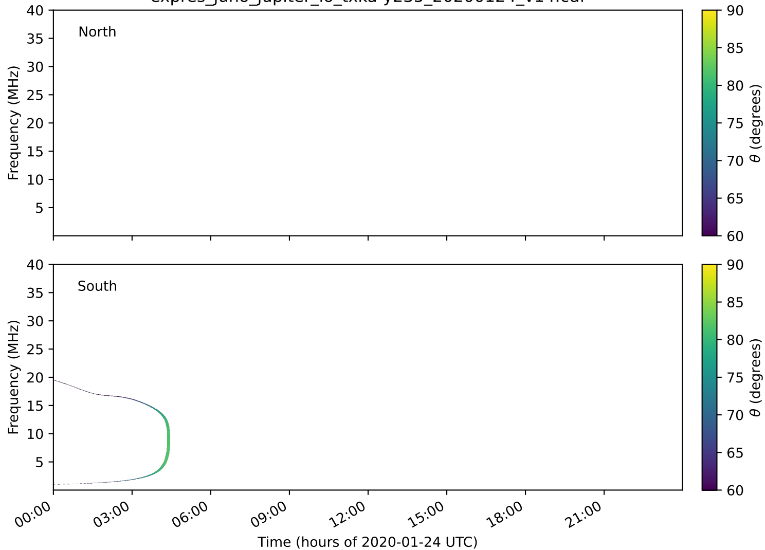
expres_juno_jupiter_io_txka-y235_20200124_v14.cdf
