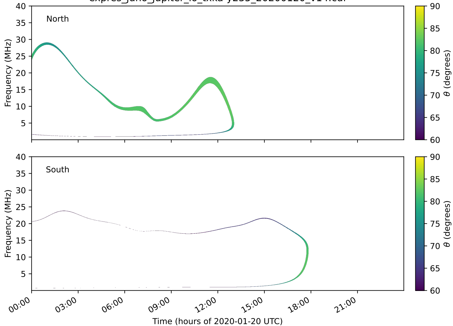
expres_juno_jupiter_io_txka-y235_20200120_v14.cdf
