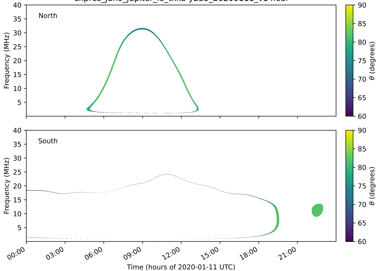
expres_juno_jupiter_io_txka-y235_20200111_v14.cdf
