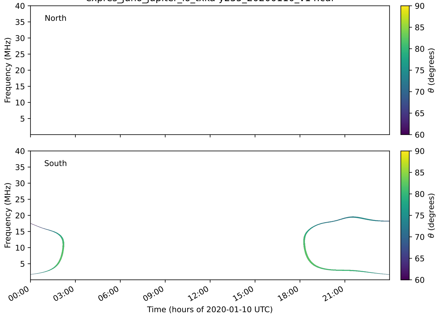
expres_juno_jupiter_io_txka-y235_20200110_v14.cdf
