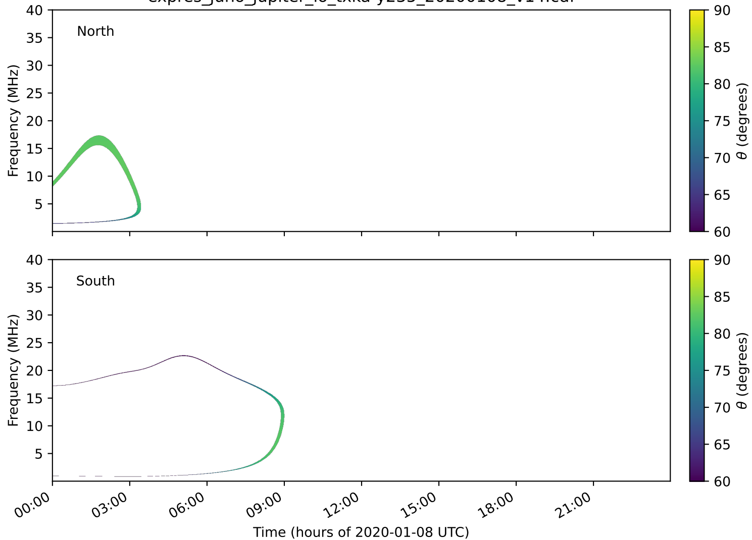
expres_juno_jupiter_io_txka-y235_20200108_v14.cdf
