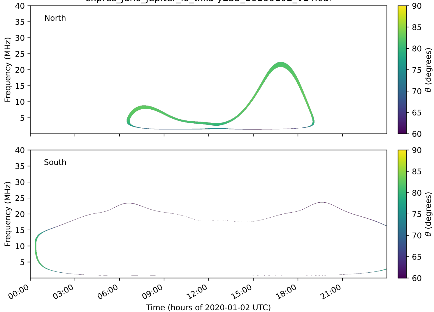
expres_juno_jupiter_io_txka-y235_20200102_v14.cdf
