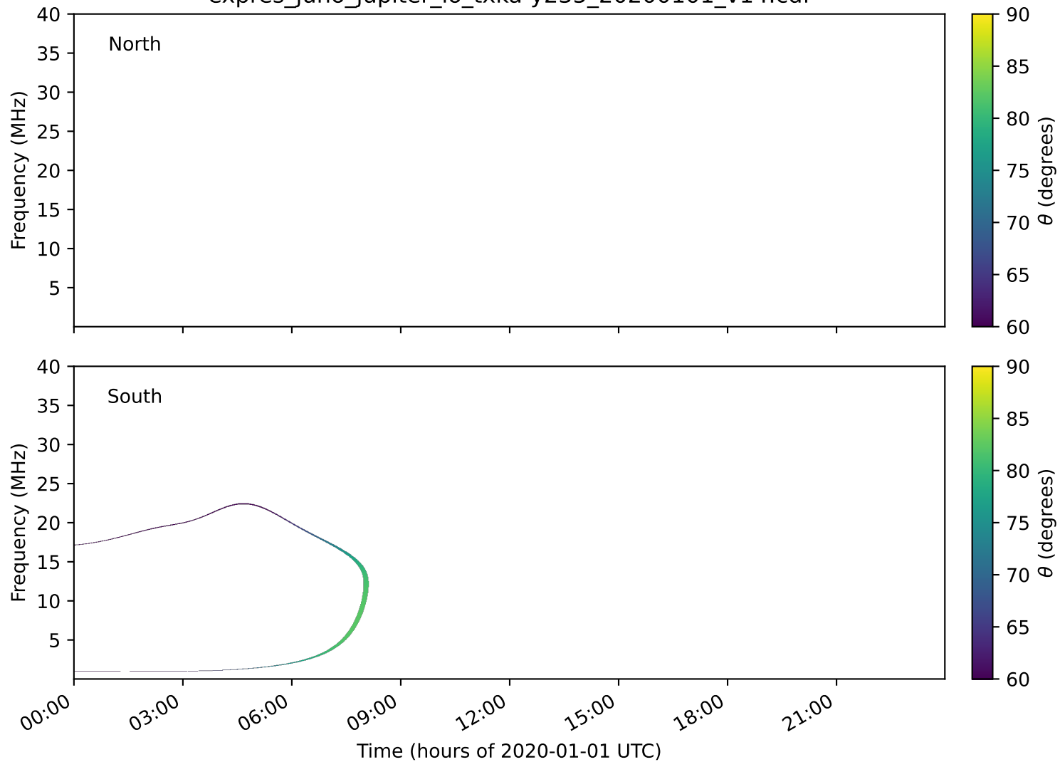
expres_juno_jupiter_io_txka-y235_20200101_v14.cdf
