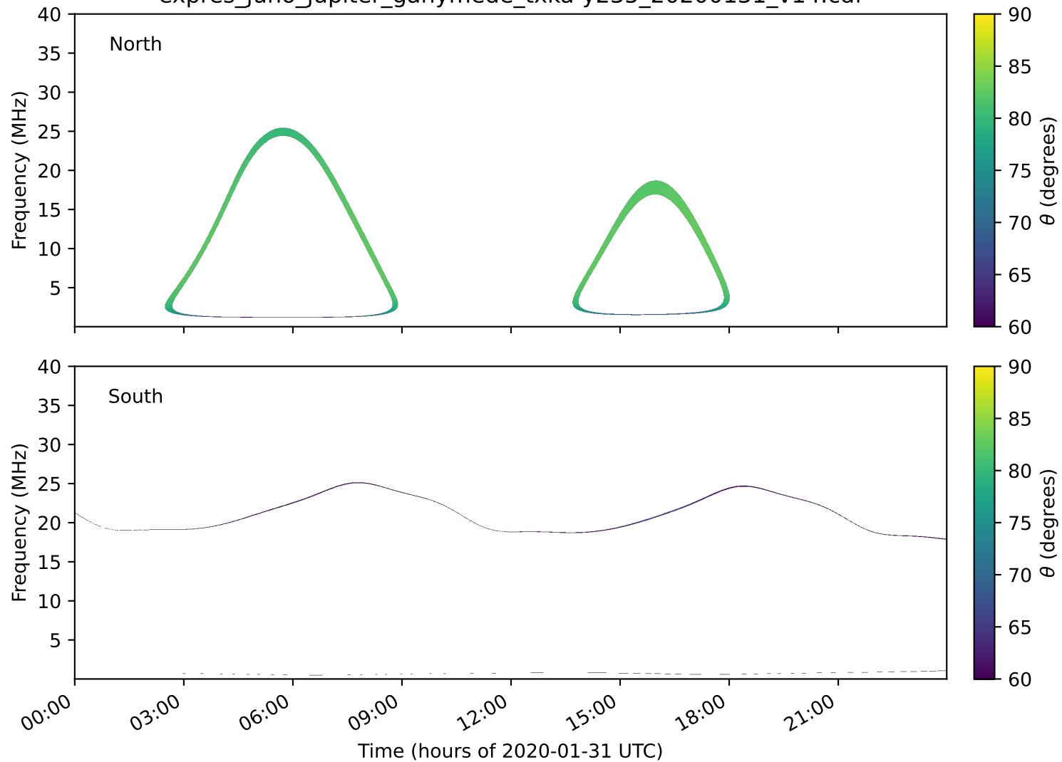
expres_juno_jupiter_ganymede_txka-y235_20200131_v14.cdf
