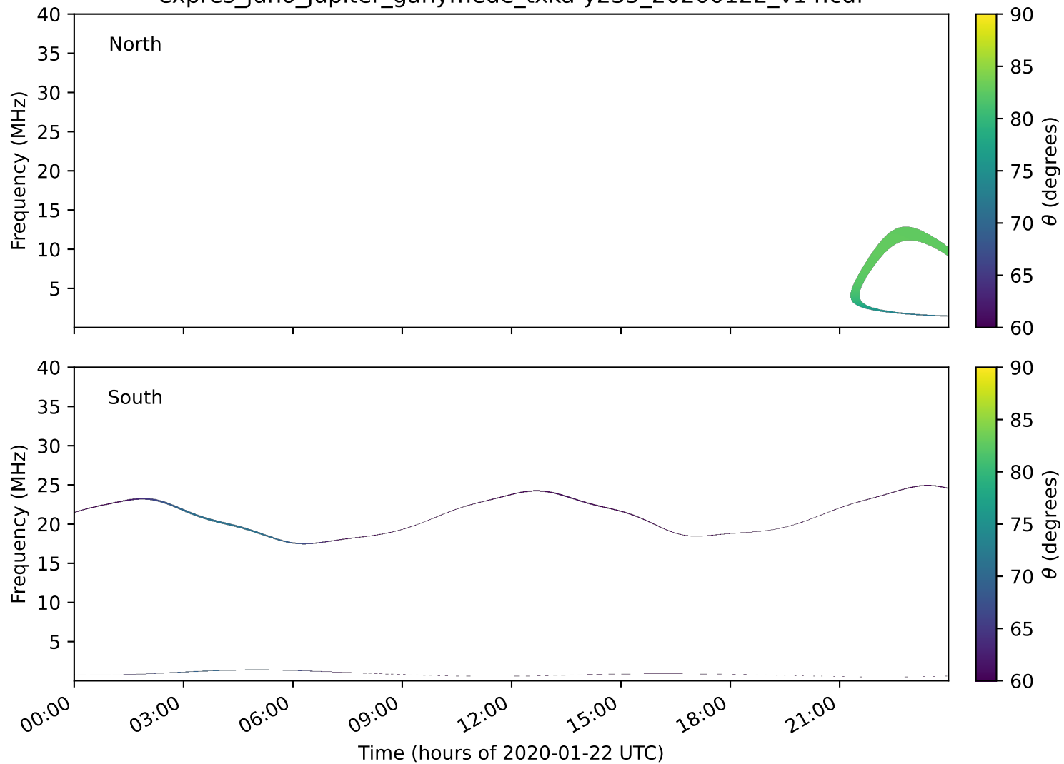
expres_juno_jupiter_ganymede_txka-y235_20200122_v14.cdf
