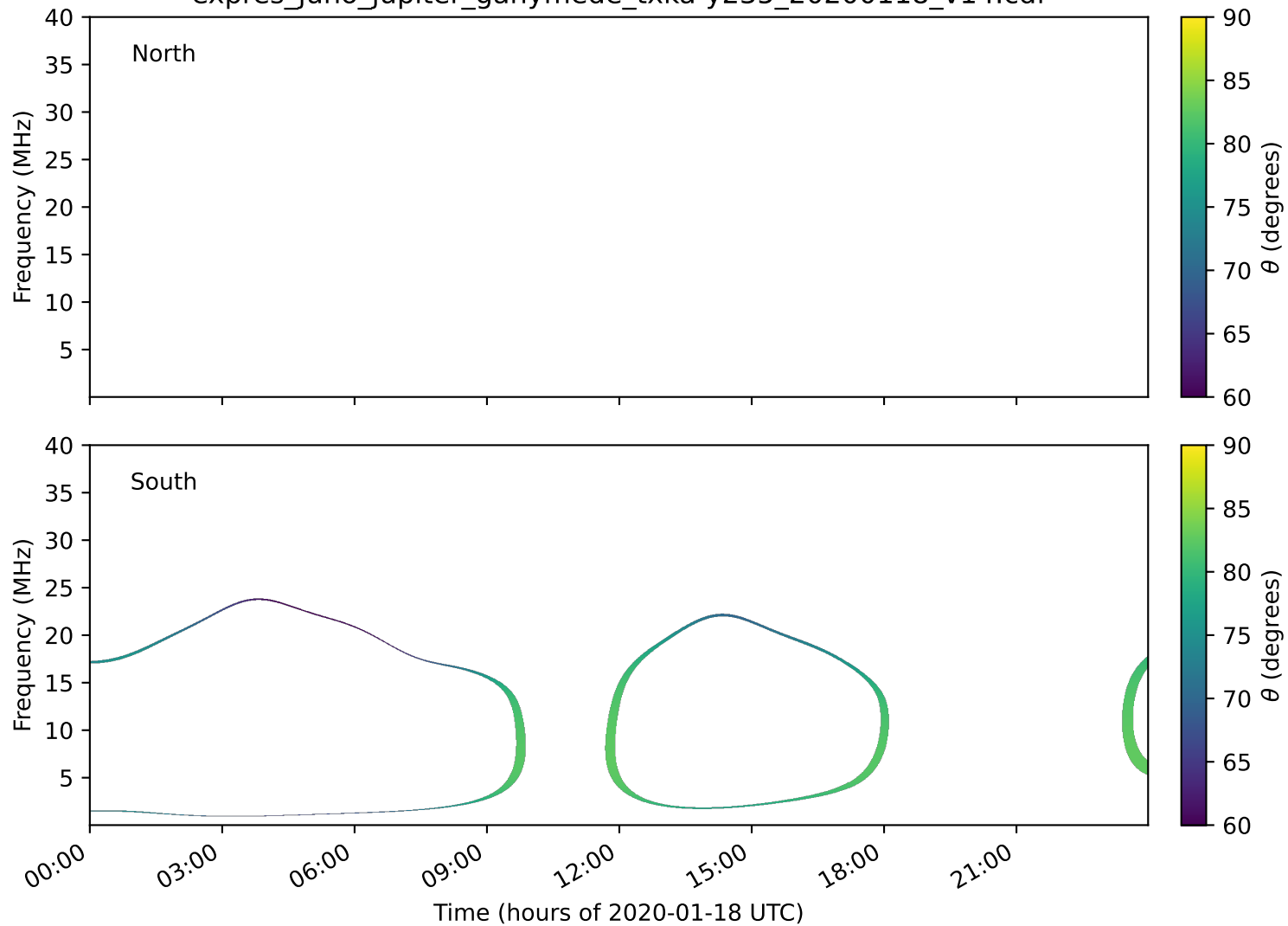
expres_juno_jupiter_ganymede_txka-y235_20200118_v14.cdf
