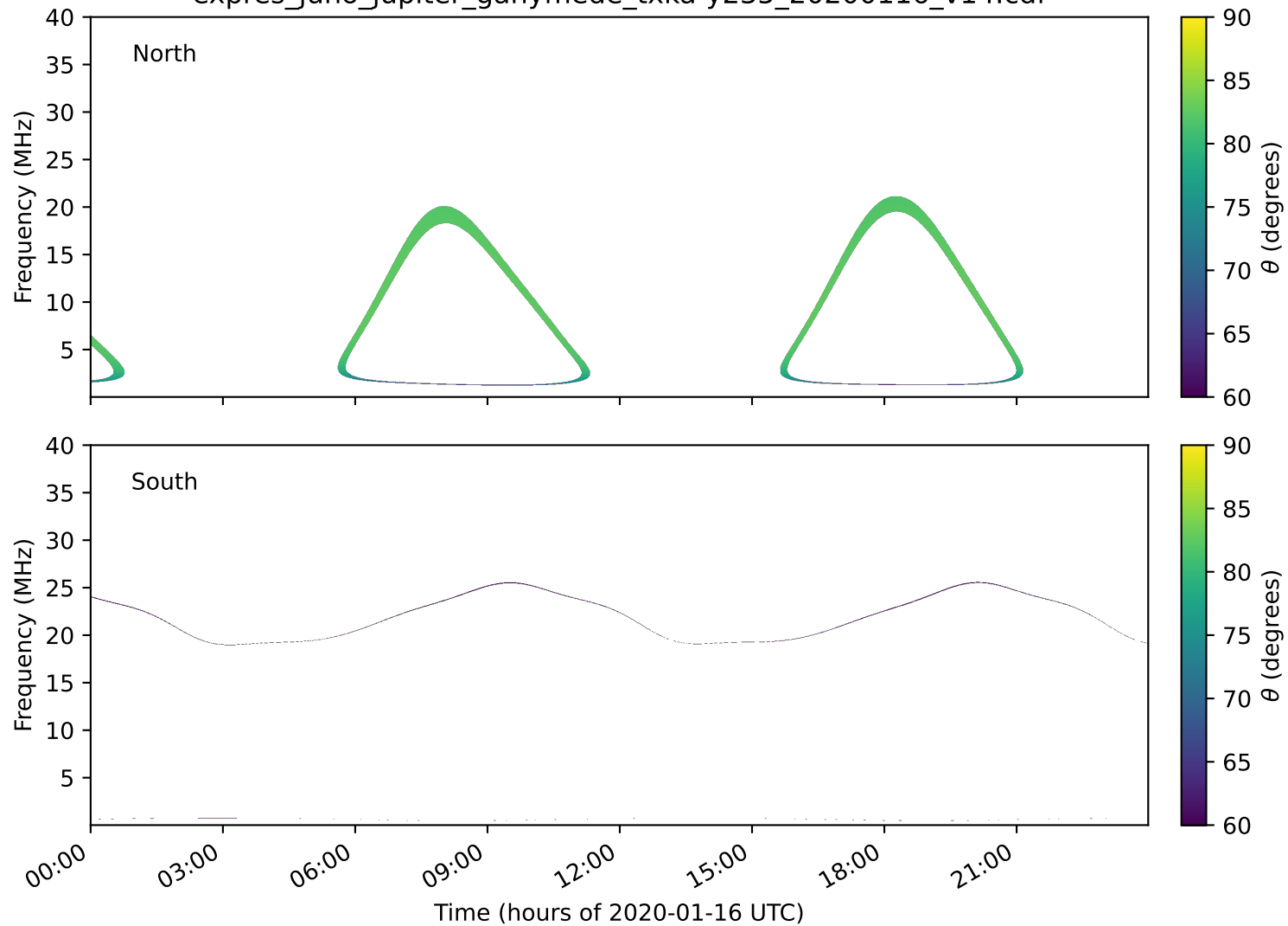
expres_juno_jupiter_ganymede_txka-y235_20200116_v14.cdf
