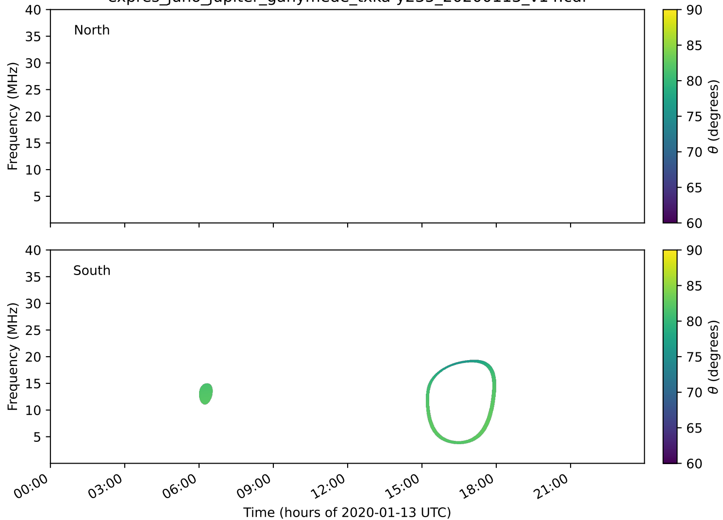
expres_juno_jupiter_ganymede_txka-y235_20200113_v14.cdf
