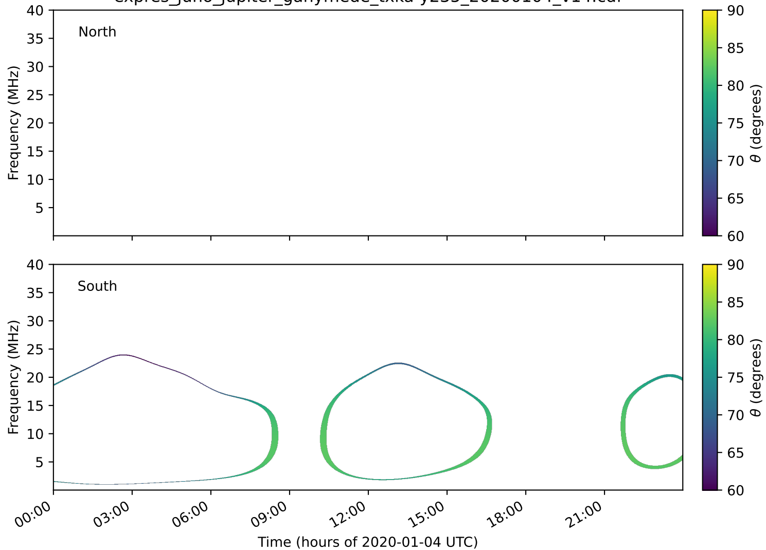
expres_juno_jupiter_ganymede_txka-y235_20200104_v14.cdf
