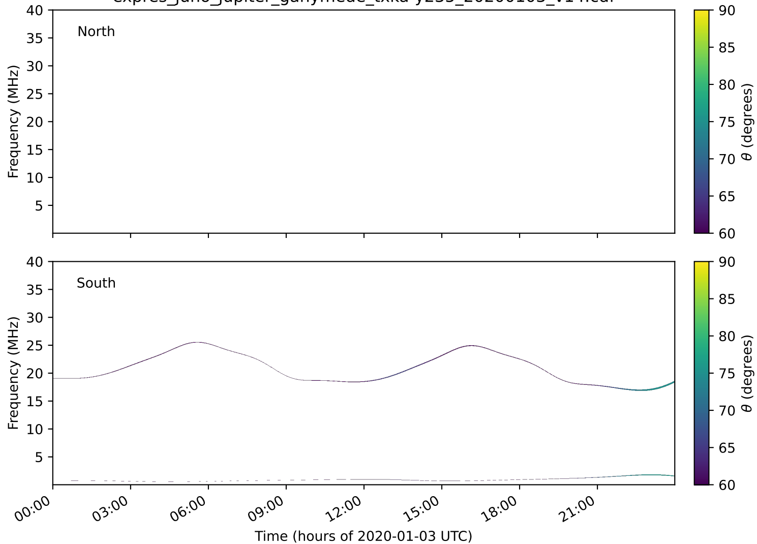
expres_juno_jupiter_ganymede_txka-y235_20200103_v14.cdf
