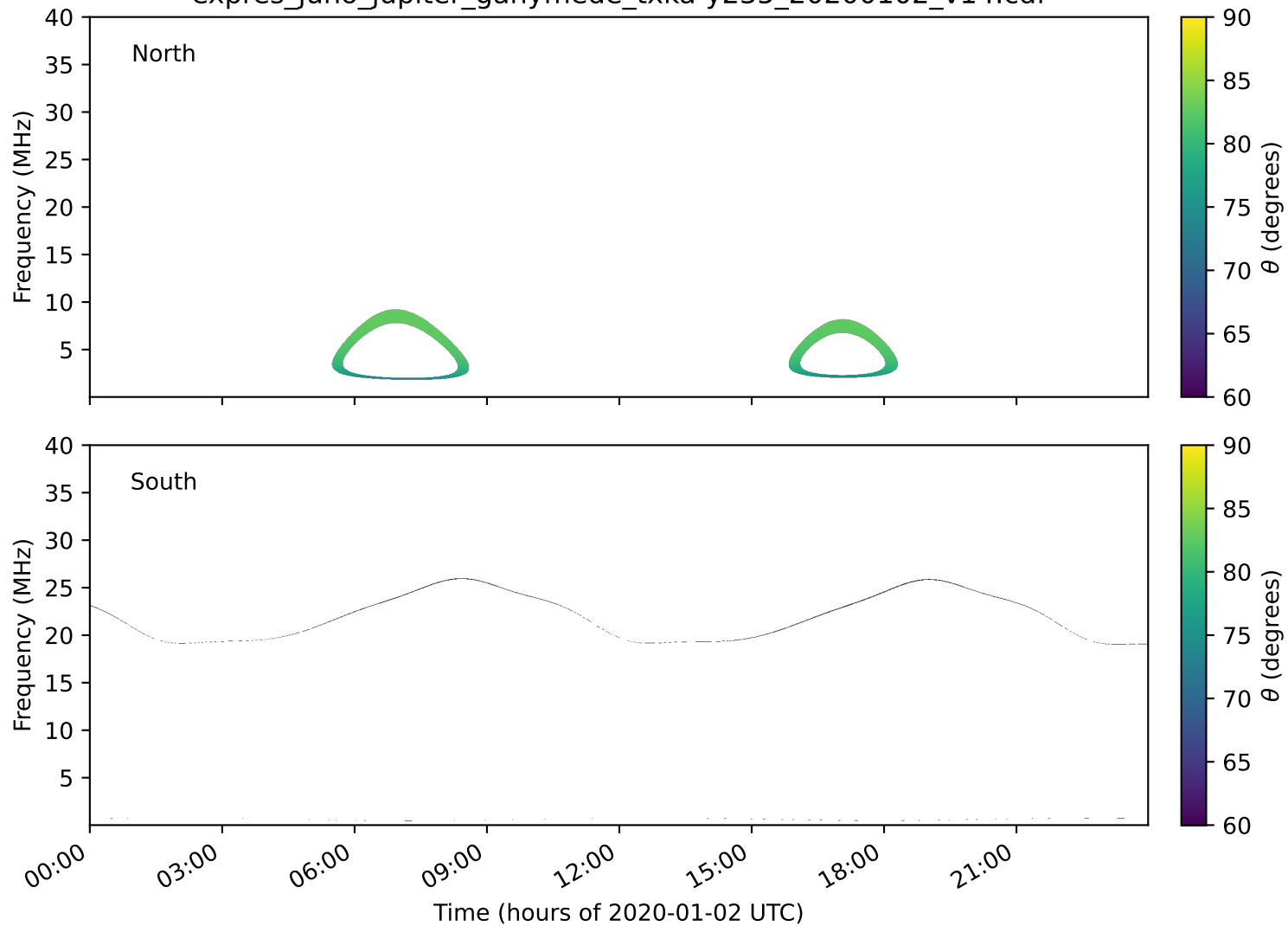
expres_juno_jupiter_ganymede_txka-y235_20200102_v14.cdf
