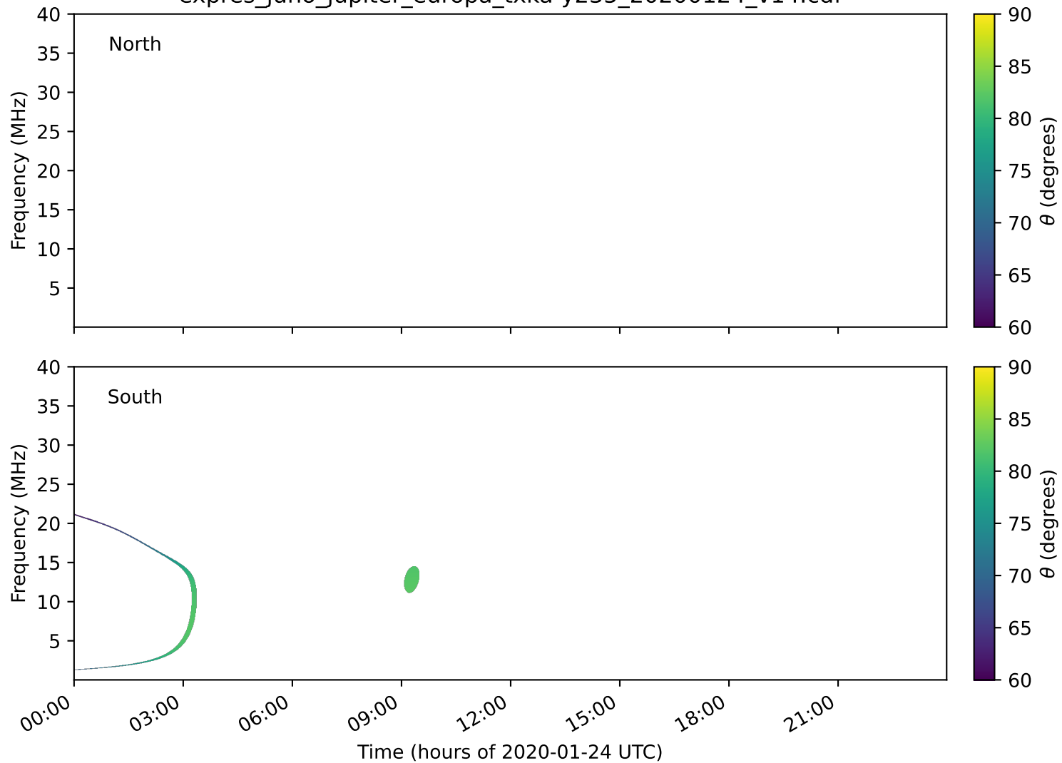
expres_juno_jupiter_europa_txka-y235_20200124_v14.cdf
