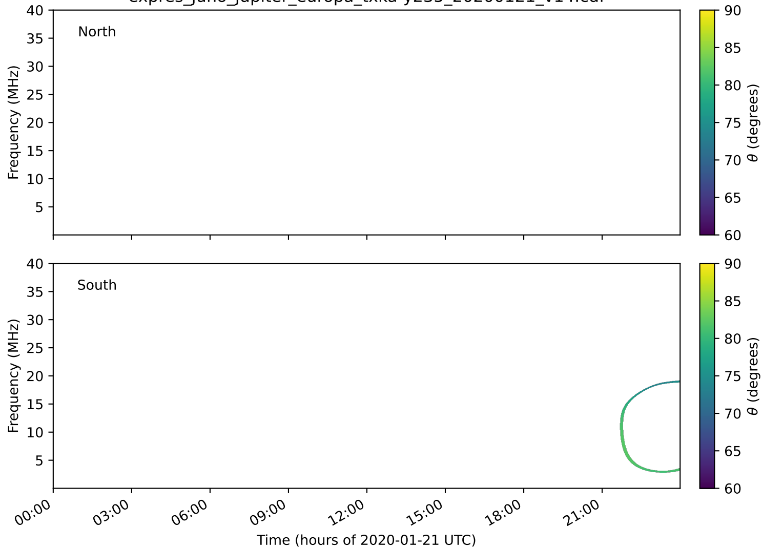
expres_juno_jupiter_europa_txka-y235_20200121_v14.cdf
