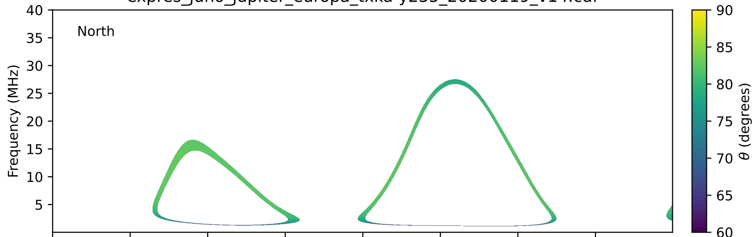
expres_juno_jupiter_europa_txka-y235_20200119_v14.cdf
