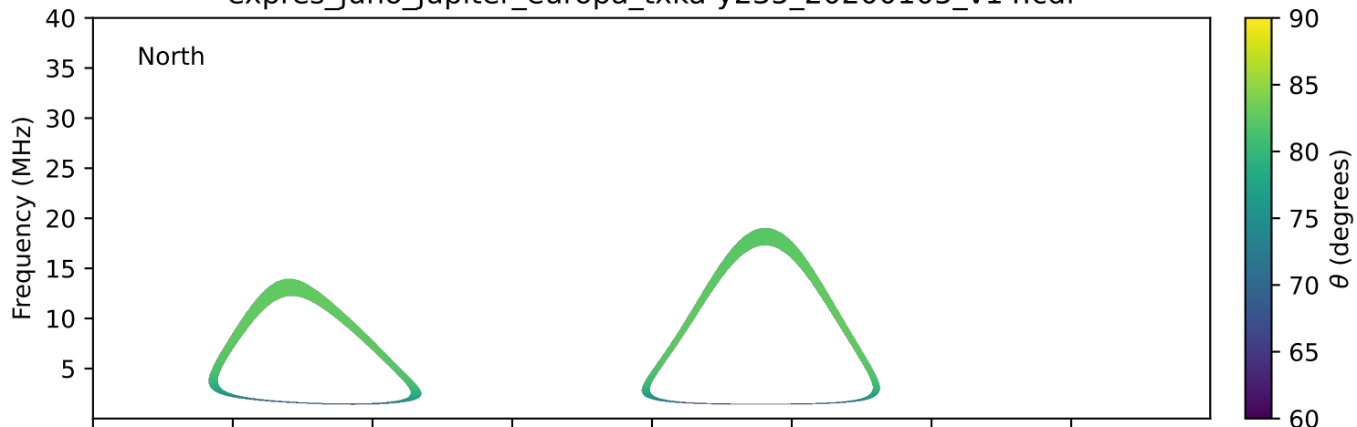
expres_juno_jupiter_europa_txka-y235_20200105_v14.cdf
