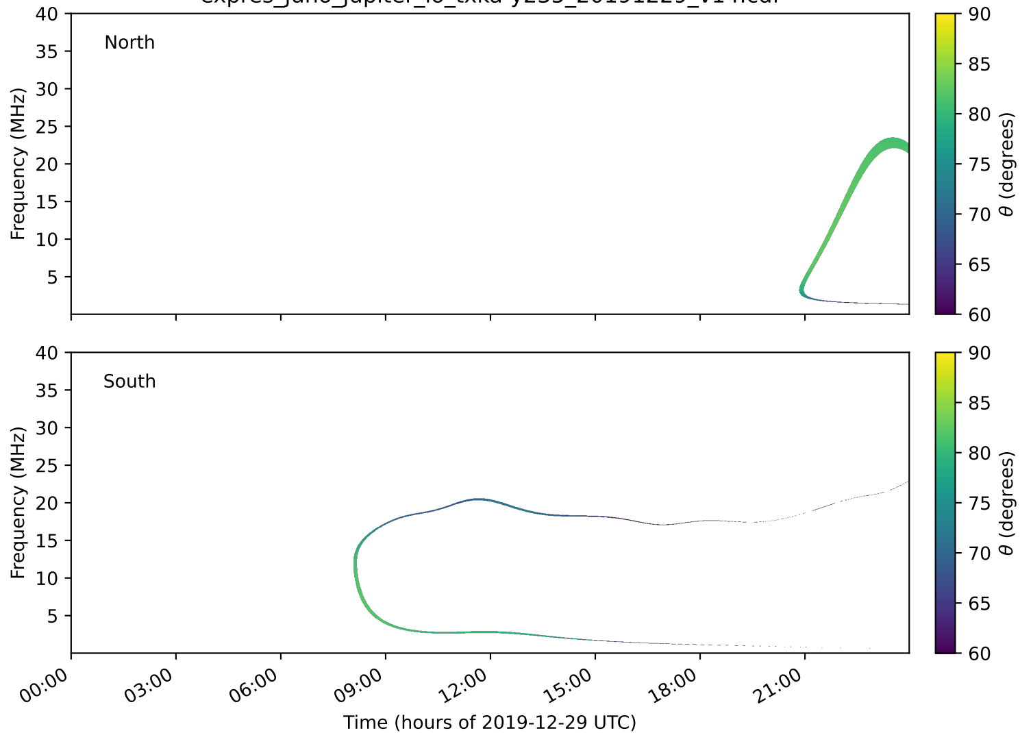
expres_juno_jupiter_io_txka-y235_20191229_v14.cdf
