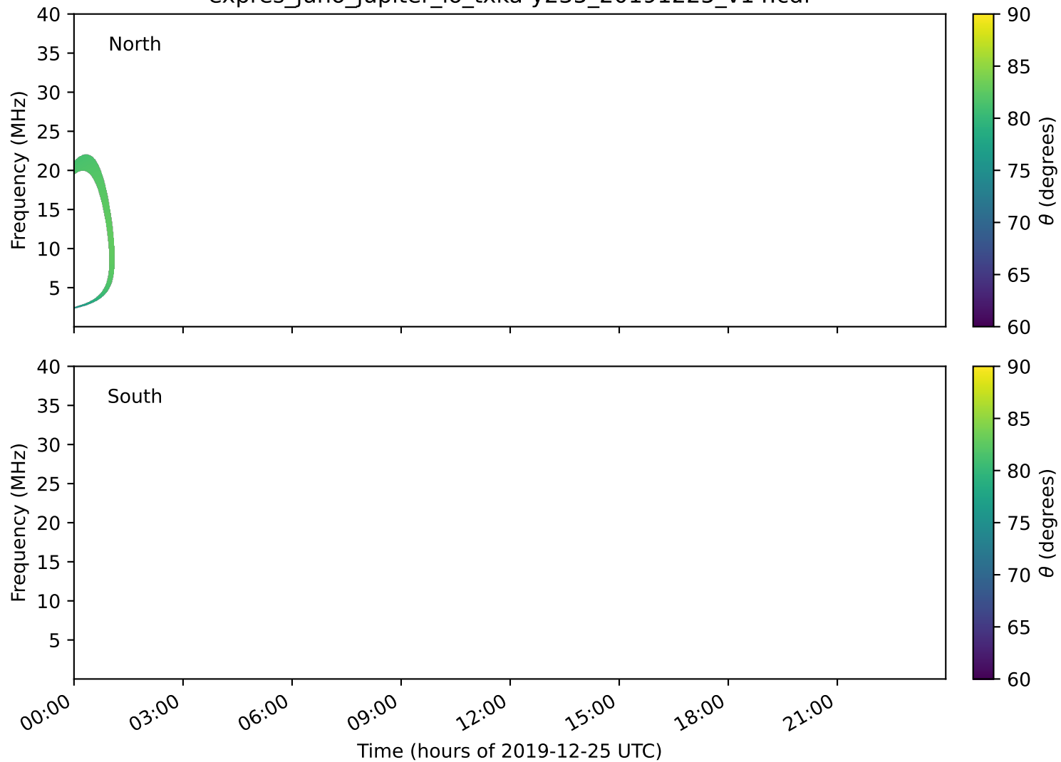
expres_juno_jupiter_io_txka-y235_20191225_v14.cdf
