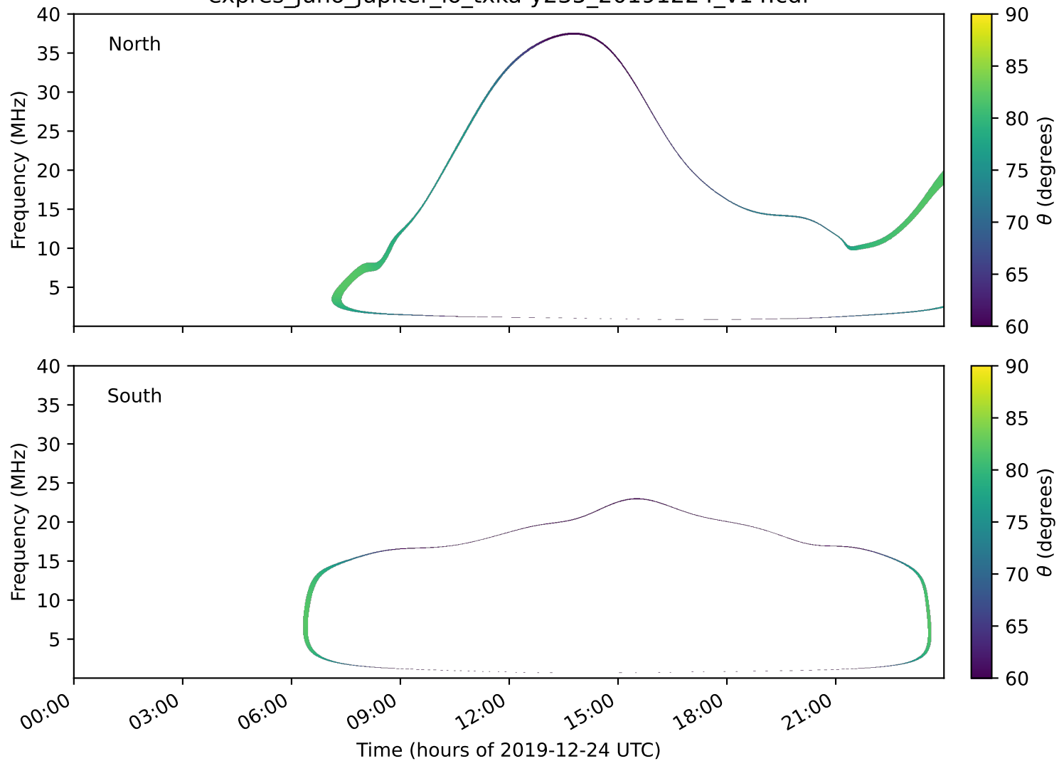
expres_juno_jupiter_io_txka-y235_20191224_v14.cdf
