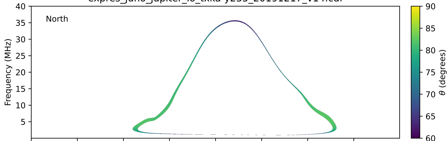
expres_juno_jupiter_io_txka-y235_20191217_v14.cdf
