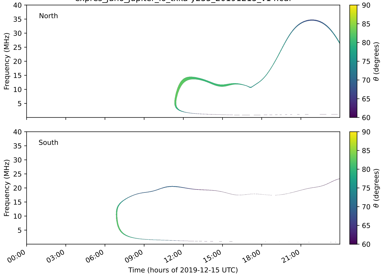
expres_juno_jupiter_io_txka-y235_20191215_v14.cdf
