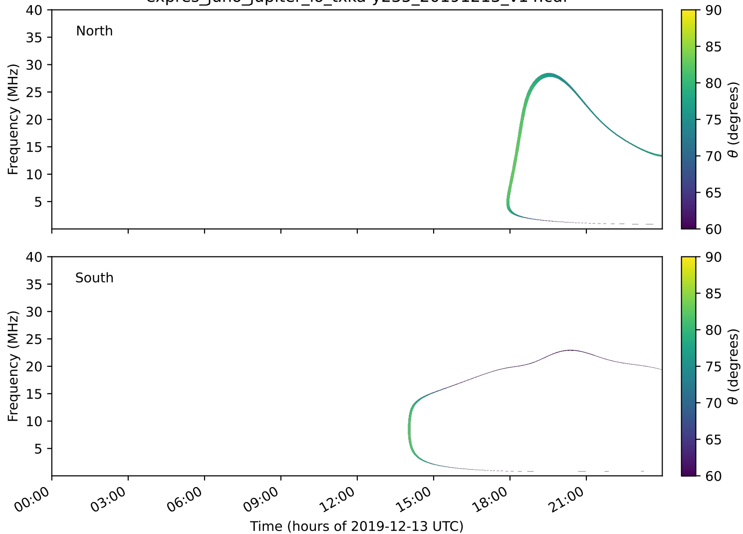
expres_juno_jupiter_io_txka-y235_20191213_v14.cdf
