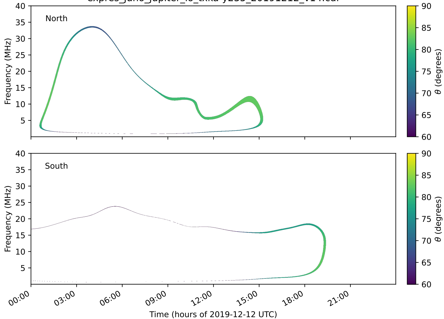
expres_juno_jupiter_io_txka-y235_20191212_v14.cdf
