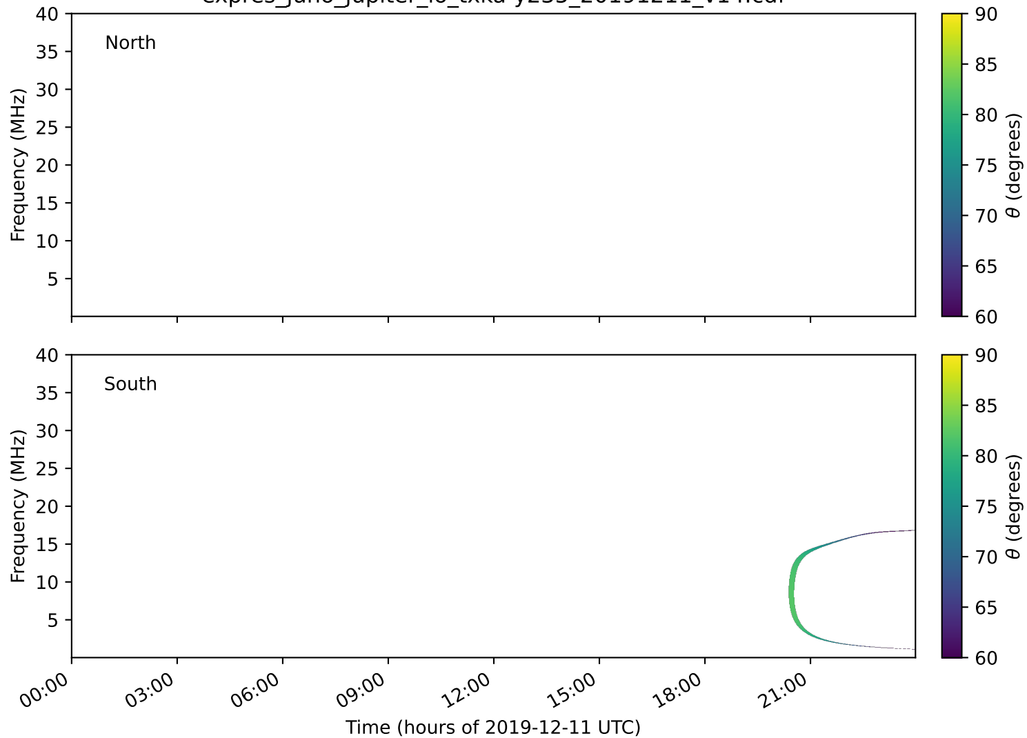
expres_juno_jupiter_io_txka-y235_20191211_v14.cdf
